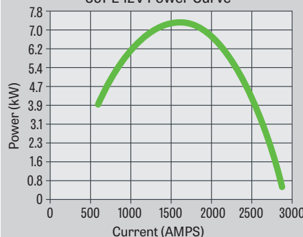
39PE 12V Power Curve
